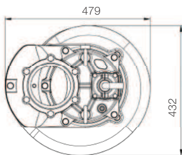
Opened Impeller
